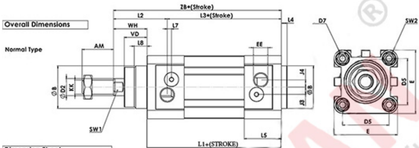
Dimension Sheet
